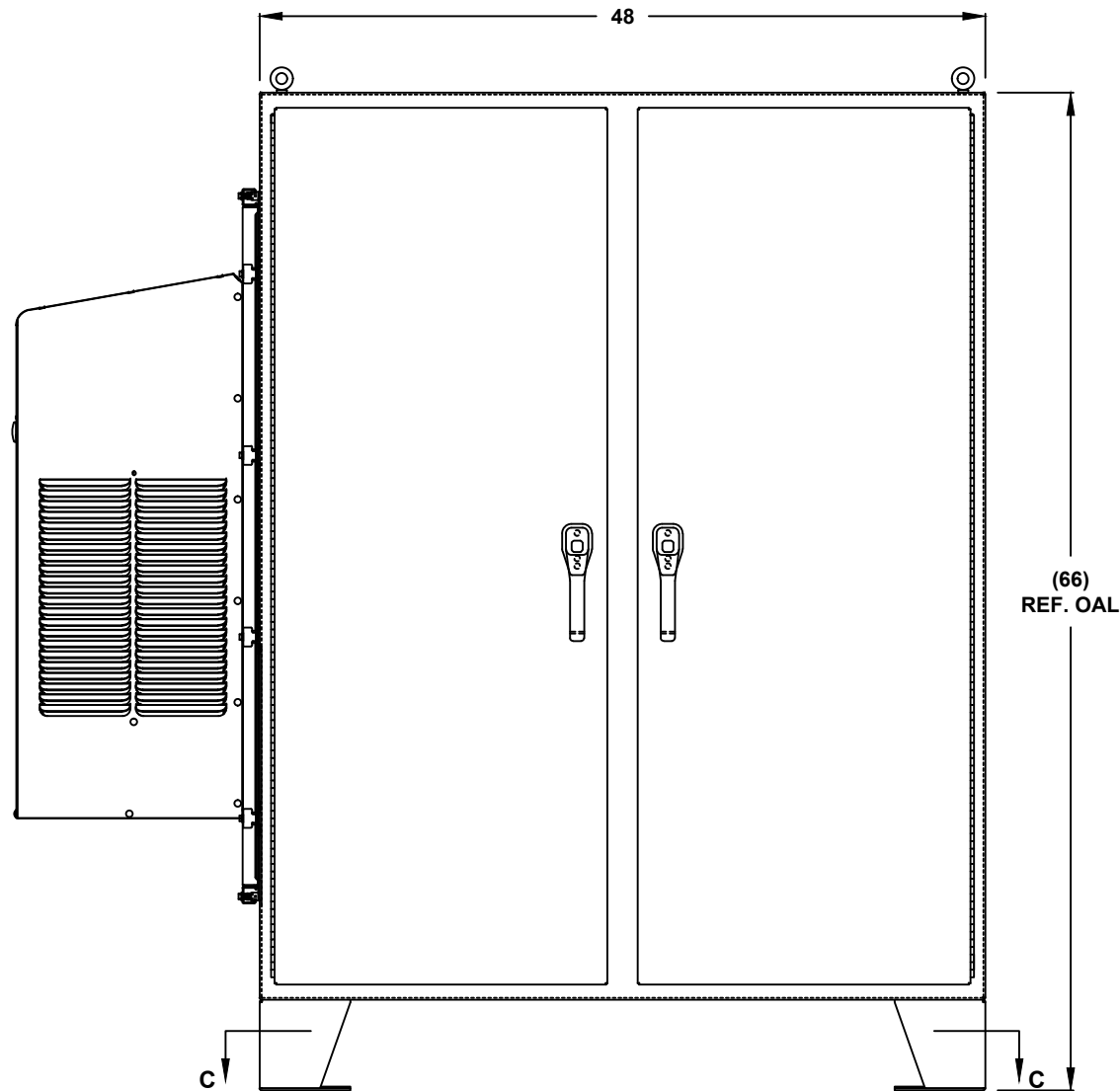
FRONT VIEW
